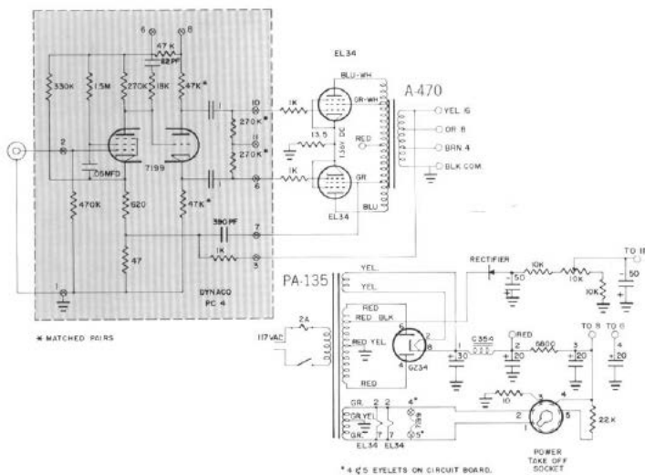
DYNAKIT MARK IV 40 WATT POWER AMPLIFIER
