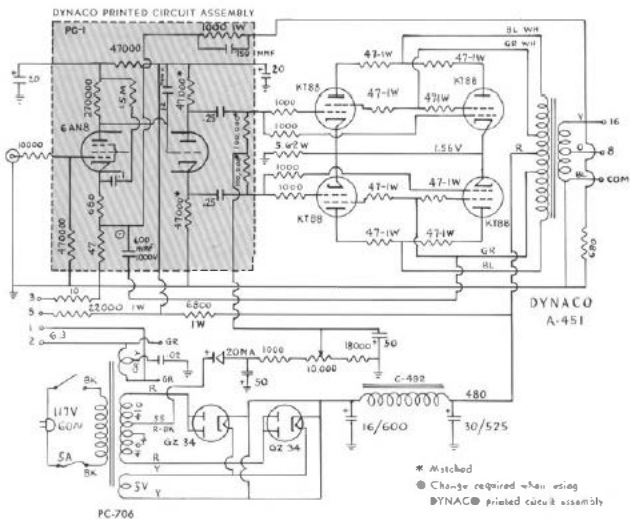
DYNACO 120 WATT AMPLIFIER USING DYNACO A-451 TRANSFORMER
