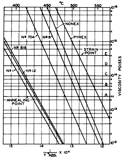
Fig. 4 - Viscosity of glasses between annealing and strain points. The intersection of lines A, B, C, and E with the viscosity curves for the various glasses indicate the temperature intervals at which the viscosities are doubled, as shown in the tabulation immediately preceding Table II.
