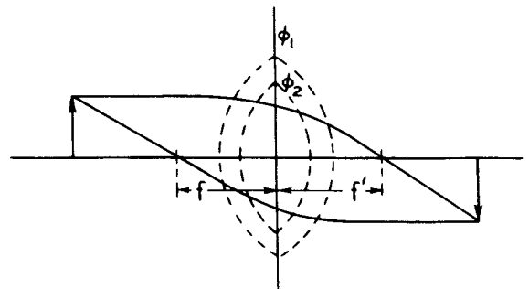
Fig. 8 - Doubler-layer lens.
