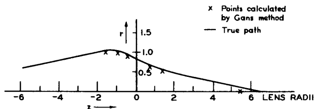
Fig. 13 - Electron trajectory through cylinder lens.
