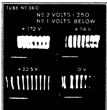
Fig. 8 - Beam traces on an anode. (Courtesy of The Institute of Radio Engineers)
