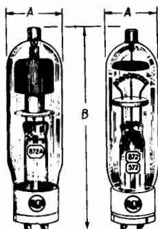
Overall Dimensions
