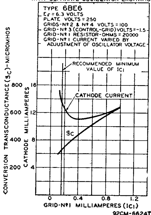
OPERATION CHARACTERISTICS WITH SEPARATE OSCILLATOR EXCITATION
