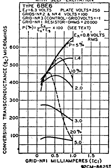
OPERATION CHARACTERISTICS WITH SELF-EXCITATION
