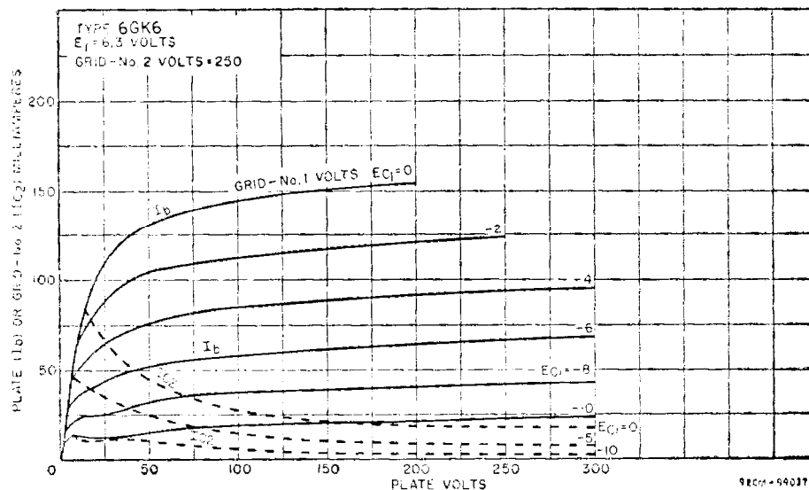
AVERAGE CHARACTERISTICS
