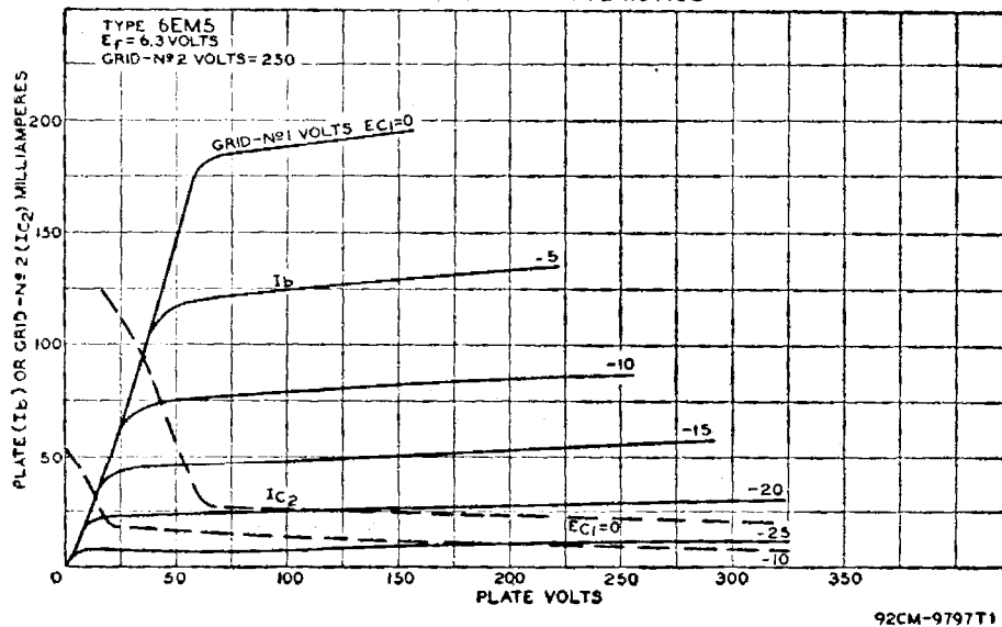
AVERAGE CHARACTERISTICS
