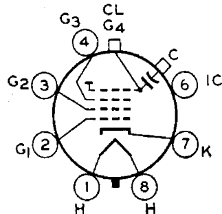
8JR ULTOR = G_4 + CL FOCUSING ELECTRODE = G_3
