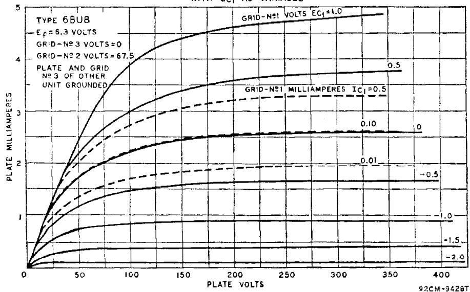
AVERAGE CHARACTERISTICS WITH E_{C1} AS VARIABLE
