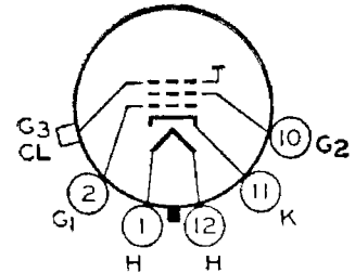
12D ULTOR = G_3 + CL
