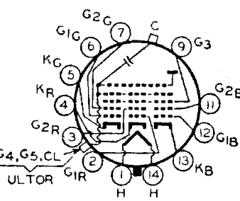
14AU ULTOR = G_4 + G_5 + CL FOCUSING ELECTRODE = G_3
