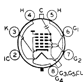
8KP ULTOR = G_3 + G_5 + CL FOCUSING ELECTRODE = G_4
