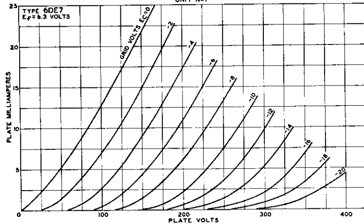
AVERAGE PLATE CHARACTERISTICS UNIT No.2
