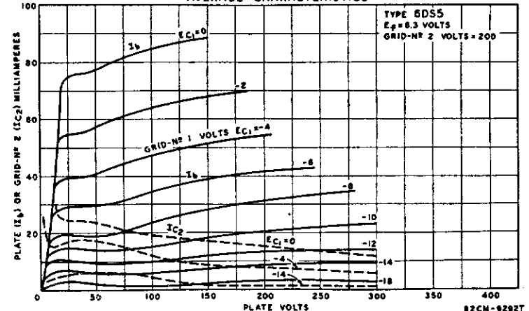
AVERAGE CHARACTERISTICS
