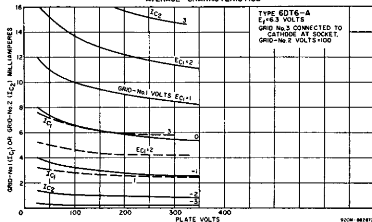
AVERAGE CHARACTERISTICS
