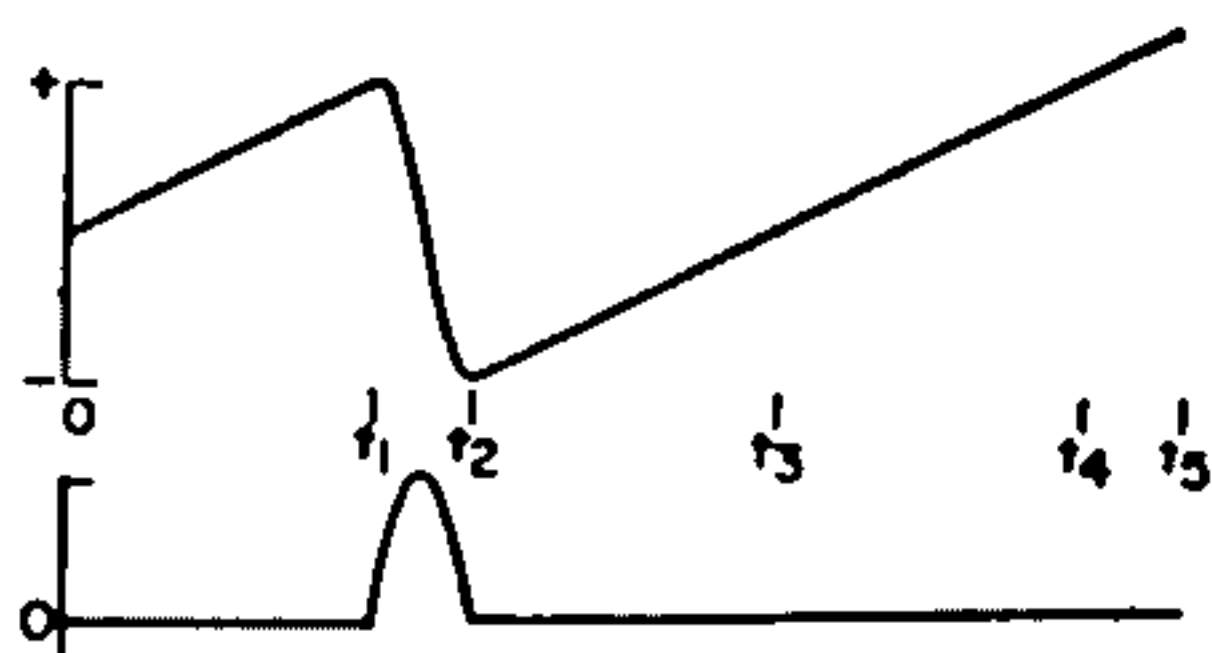
Fig. 87—Yoke-current (upper) and switch-voltage (lower) waveforms when switch is closed at t_5 .
