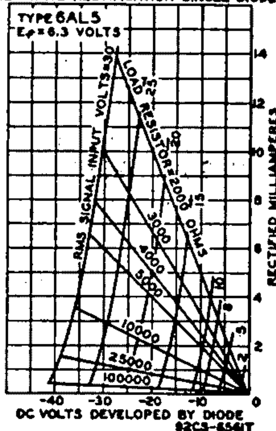
• AVERAGE CHARACTERISTICS HALF-WAVE RECTIFICATION-SINGLE DIODE
