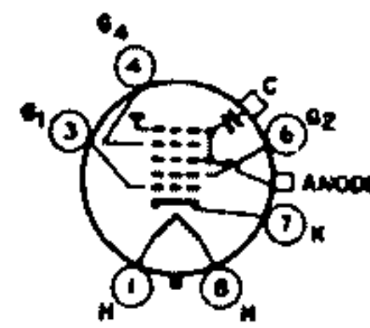
81W ANODE - G_3 + G_4 + C_1 FOCUSING ELECTRODE - G_4
