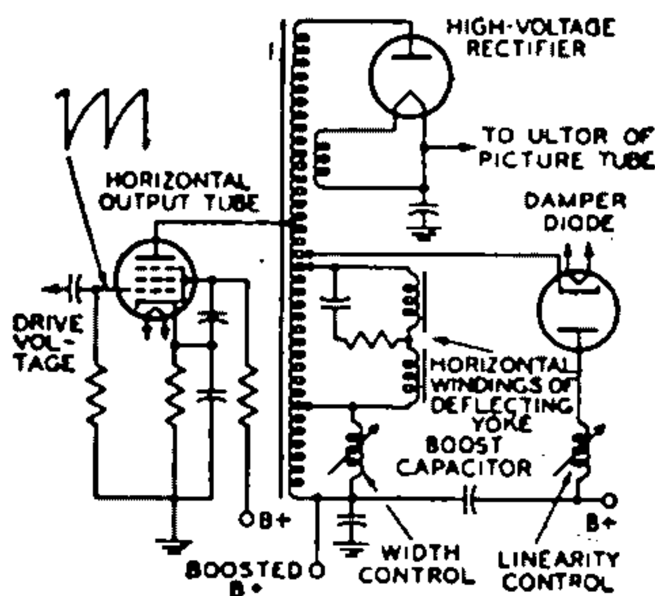
Fig. 89—Typical horizontal-deflection and high-voltage circuit.
