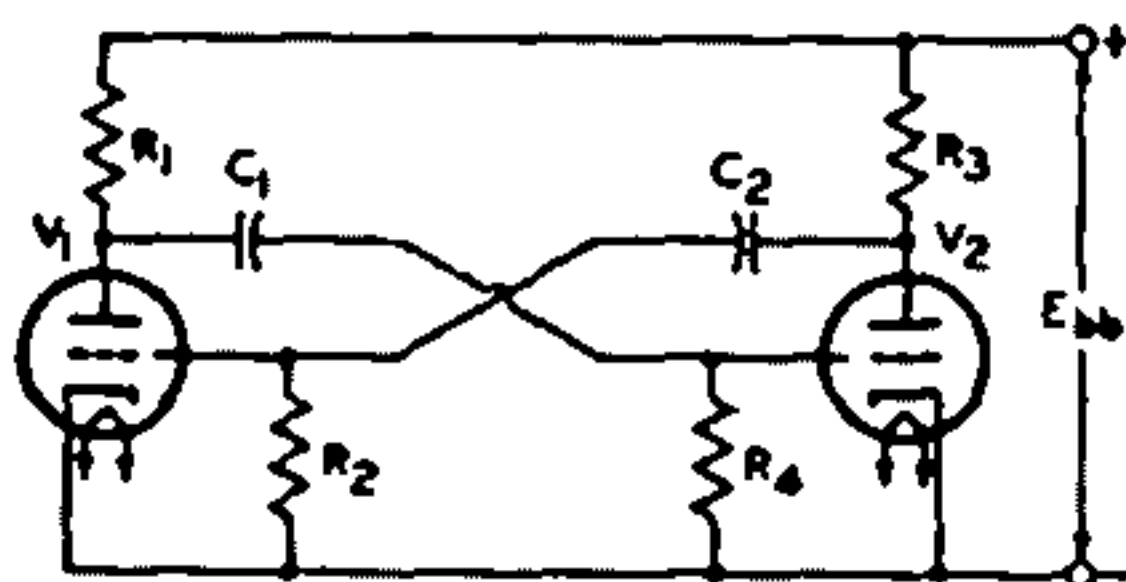
Fig. 100—Basic multivibrator circuit of the free-running type.
