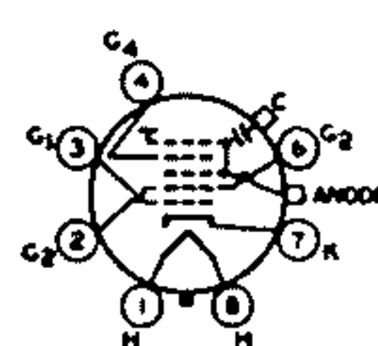
81K ANODE - G_3 + G_4 + C_1 FOCUSING ELECTRODE - G_4
