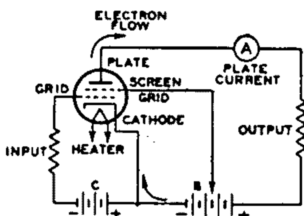
Fig. 7—Basic tetrode circuit.
