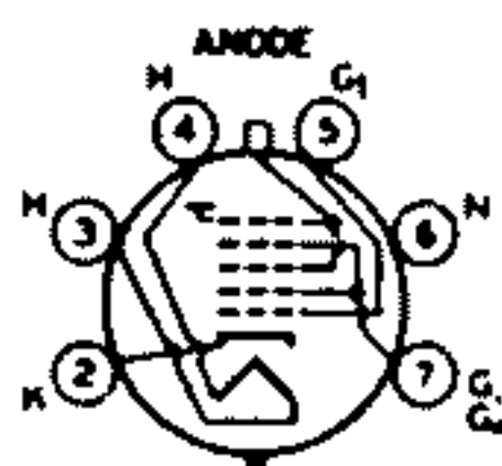
77Q ANODE - G_3 + G_4 + C_1 AUTOMATIC FOCUSING
