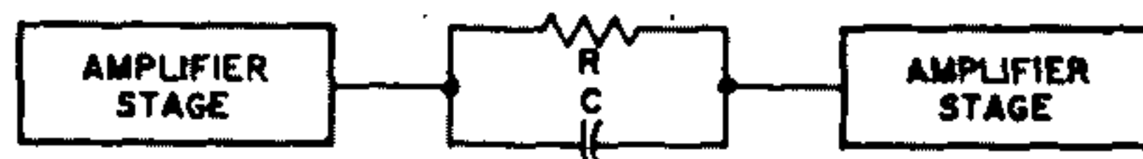
Fig. 54—Simple RC frequency-compensation network.
