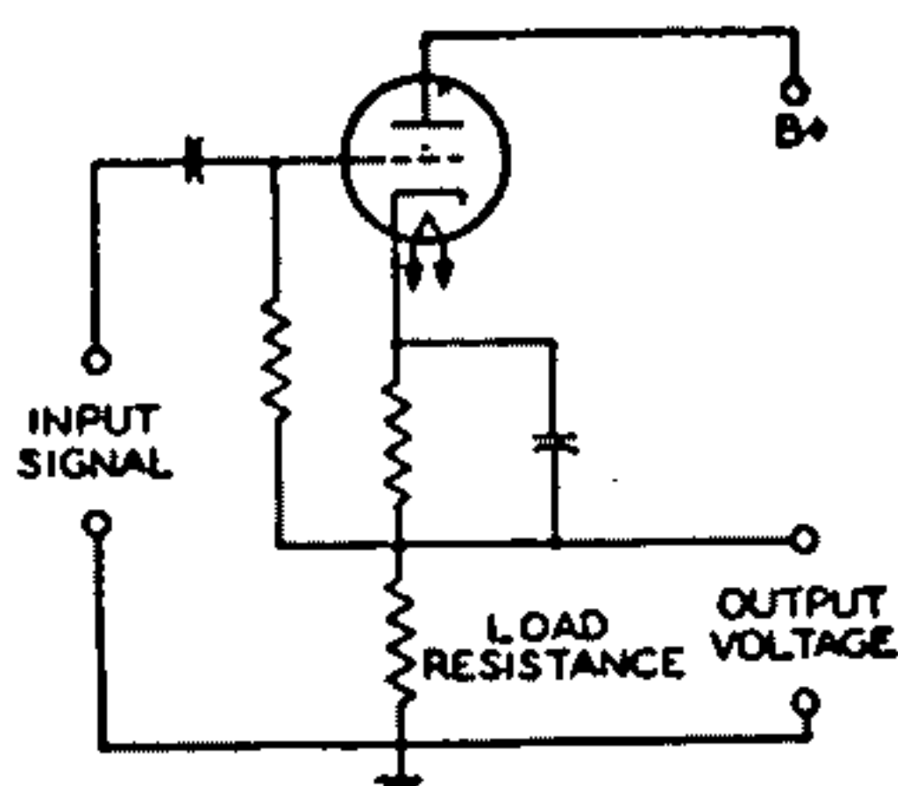
Fig. 53—Cathode-follower circuit modified for reduced bias.
