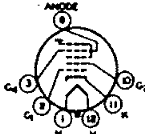
12AD ANODE - G_3 + G_4 + C_1 FOCUSING ELECTRODE - G_4
