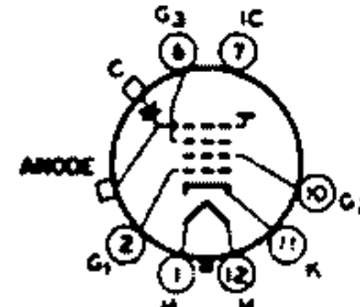
12C ANODE - G_4 + C_1 FOCUSING ELECTRODE - G_3
