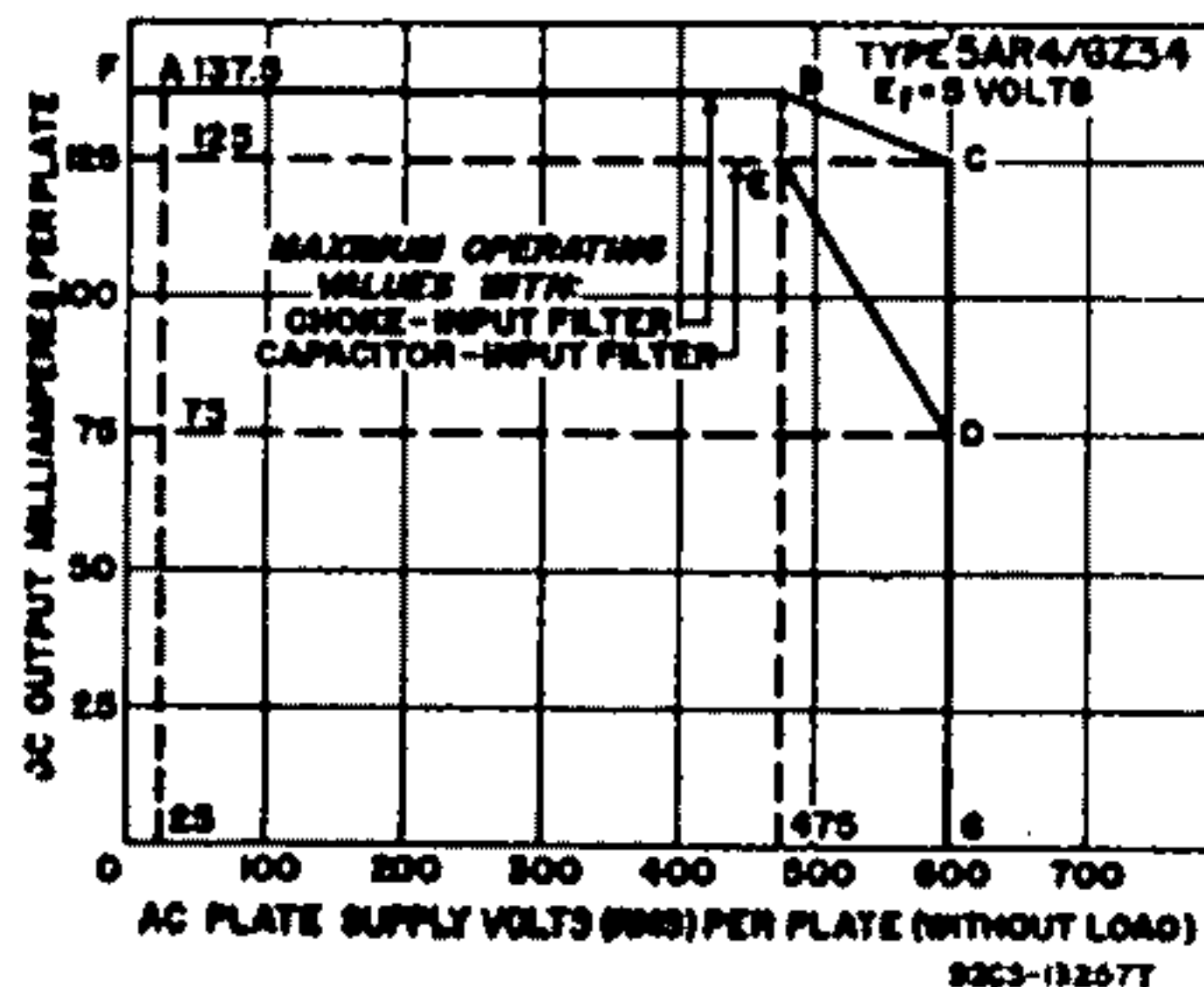
RATING CHART
