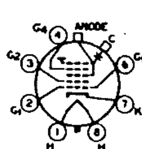
81E ANODE - G_3 + G_4 + C_1 FOCUSING ELECTRODE - G_4
