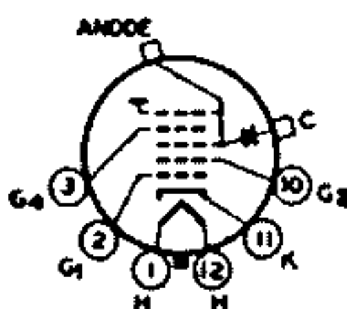
12AB ANODE - G_3 + G_4 + C_1 FOCUSING ELECTRODE - G_4
