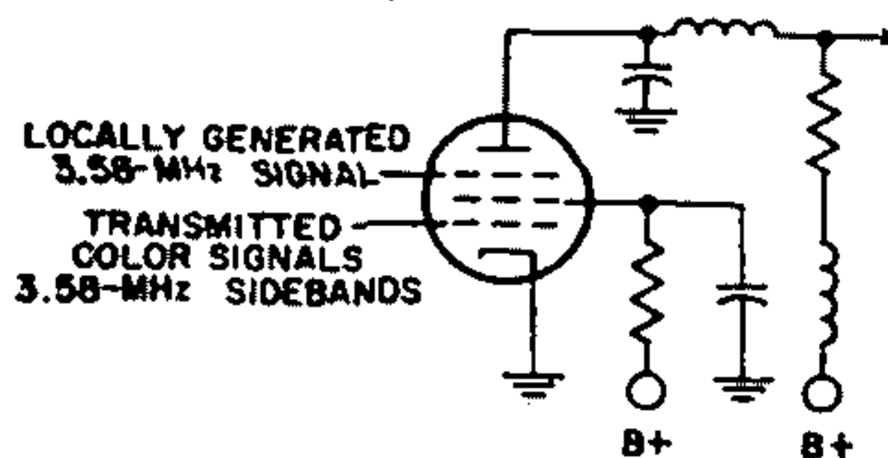
Fig. 96—Low-level color demodulator.
