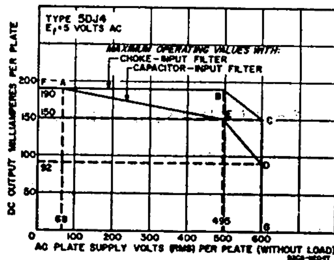
RATING CHART
