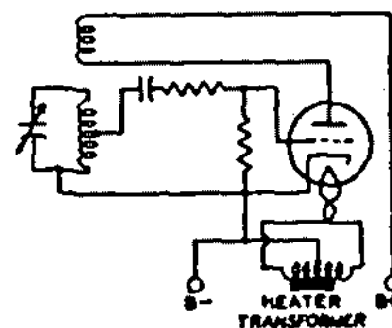
Fig. 99—Tuned-grid triode oscillator circuit using heater-cathode-type tube.
