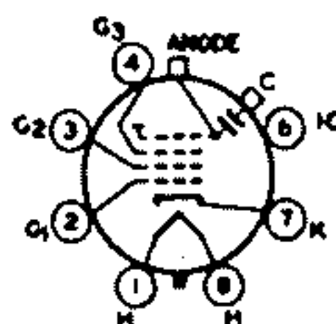
81R ANODE - G_4 + C_1 FOCUSING ELECTRODE - G_3
