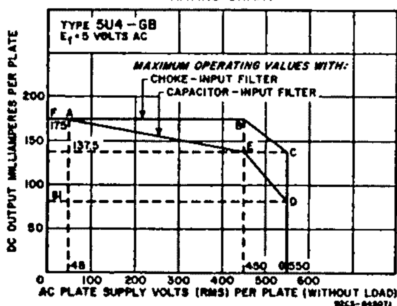
RATING CHART
