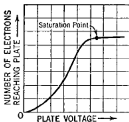
Fig. 5—Current characteristic of diode tube.
