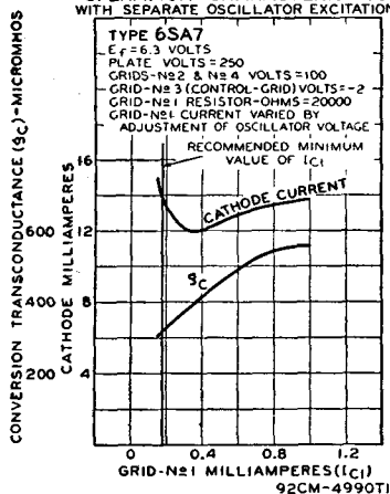
OPERATION CHARACTERISTICS WITH SEPARATE OSCILLATOR EXCITATION
