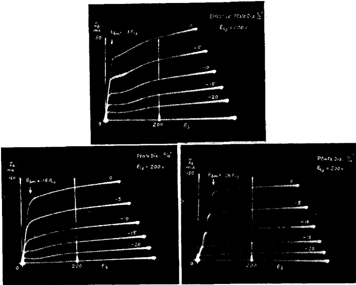
Fig. 20—Oscillograms showing plate characteristics for beam power tubes having different plate diameters.
