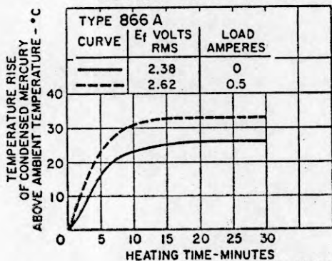
RATE OF RISE OF CONDENSED-MERCURY TEMPERATURE
