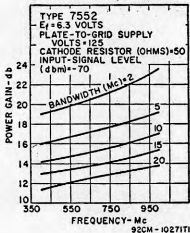
GAIN CHARACTERISTICS CATHODE-DRIVE SERVICE
