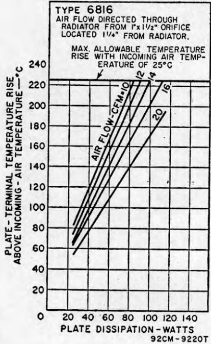
TYPICAL COOLING REQUIREMENTS
