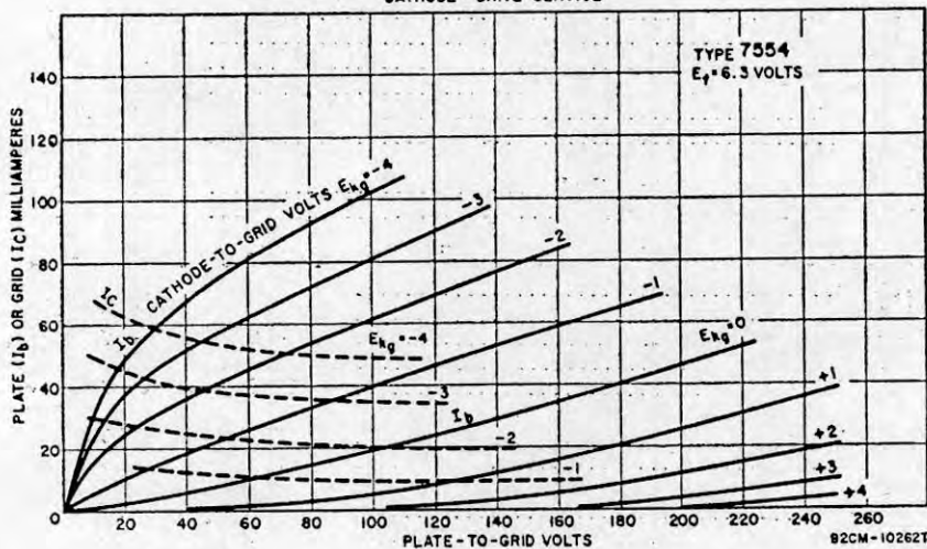
AVERAGE CHARACTERISTICS CATHODE-DRIVE SERVICE
