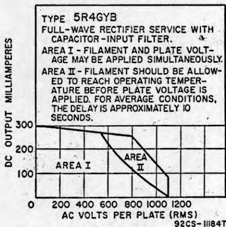
OPERATING AREAS FOR SIMULTANEOUS AND DELAYED APPLICATION OF PLATE VOLTAGE
