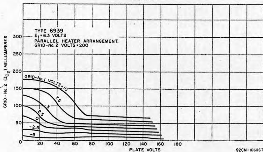
AVERAGE GRID-No. 2 CHARACTERISTICS EACH UNIT
