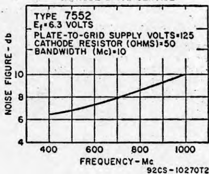
NOISE FIGURE CHARACTERISTIC CATHODE DRIVE-SERVICE
