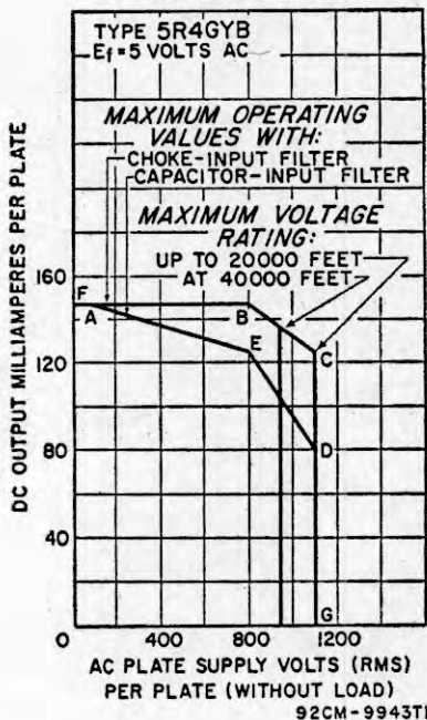
RATING CHART I
