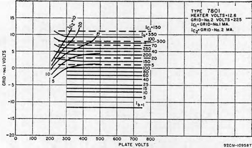
TYPICAL CONSTANT-CURRENT CHARACTERISTICS
