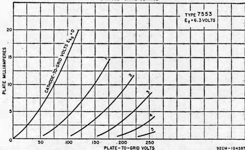
GAIN CHARACTERISTICS CATHODE-DRIVE SERVICE
