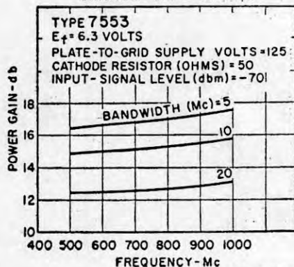
GAIN CHARACTERISTICS CATHODE-DRIVE SERVICE
