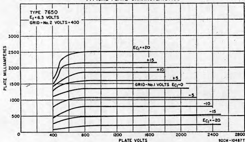
TYPICAL PLATE CHARACTERISTICS
