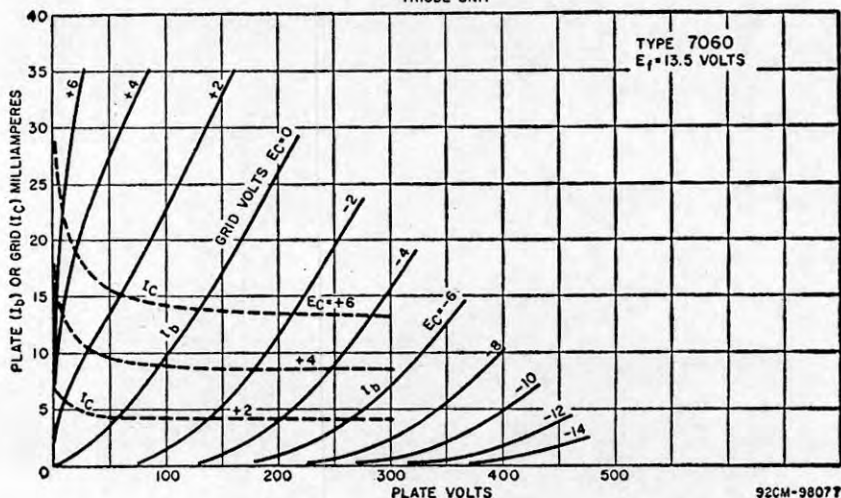
AVERAGE CHARACTERISTICS TRIODE UNIT
