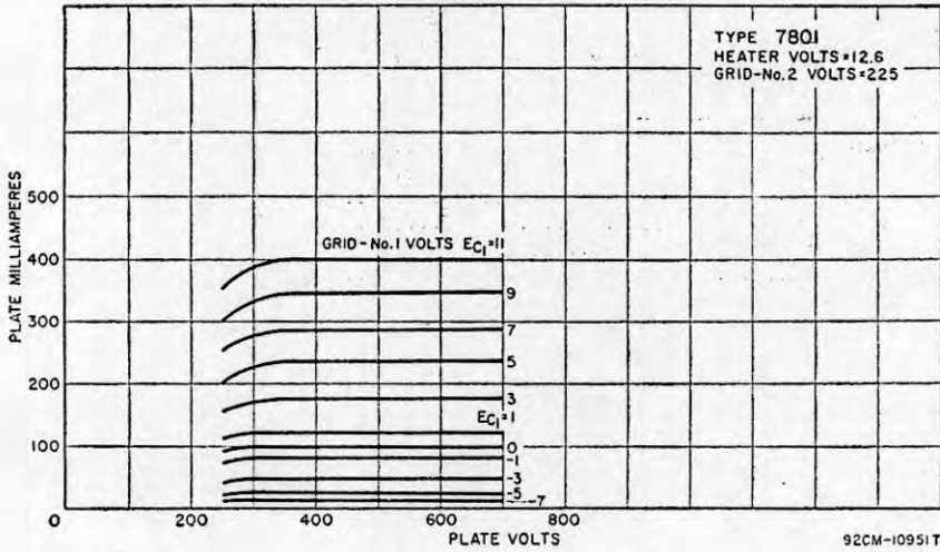
TYPICAL PLATE CHARACTERISTICS
