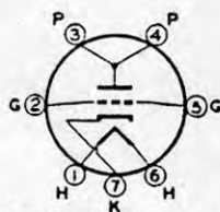
VIEWED FROM SHORT END
