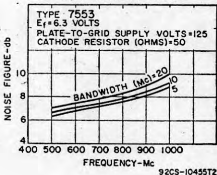
NOISE FIGURE CHARACTERISTICS CATHODE DRIVE-SERVICE
