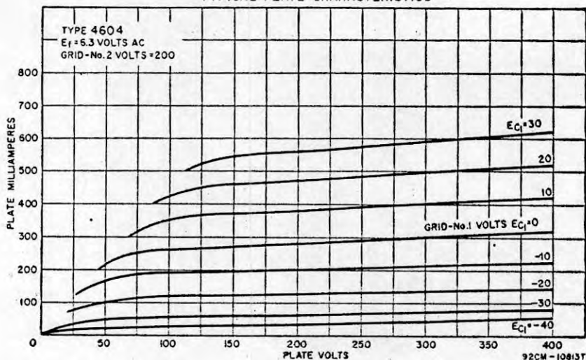
TYPICAL PLATE CHARACTERISTICS
