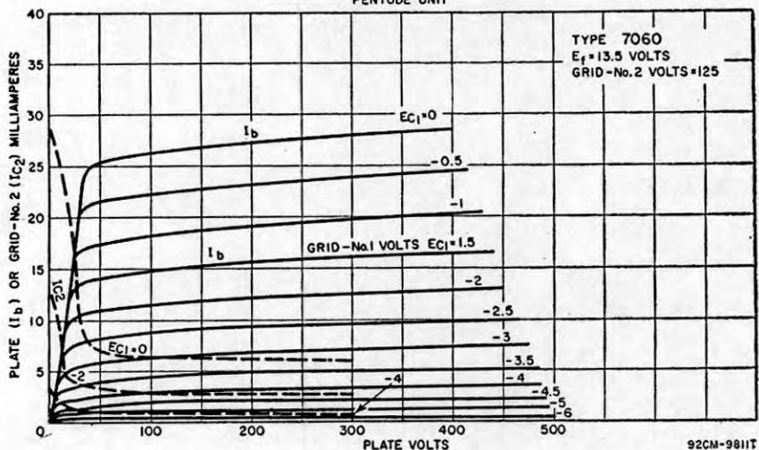
AVERAGE CHARACTERISTICS PENTODE UNIT
