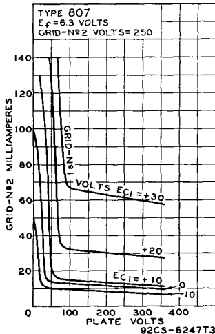
AVERAGE CHARACTERISTICS
