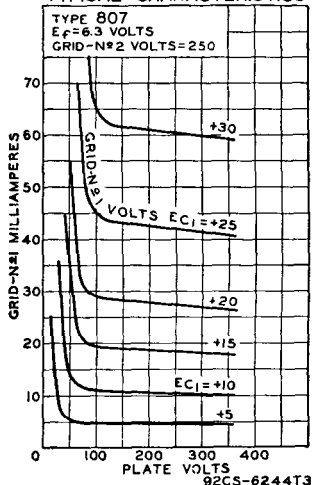
TYPICAL CHARACTERISTICS
