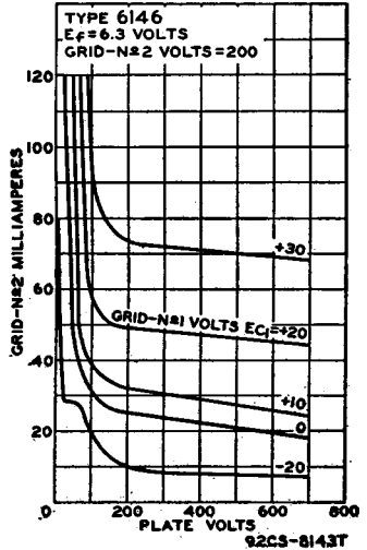
AVERAGE CHARACTERISTICS
