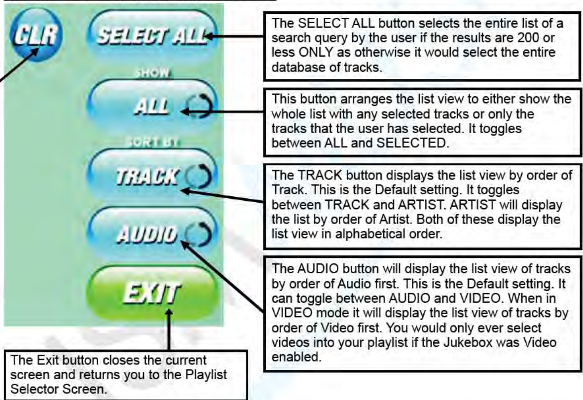
fig. 2.10.4 - Edit Playlist screen Toggle Buttons
