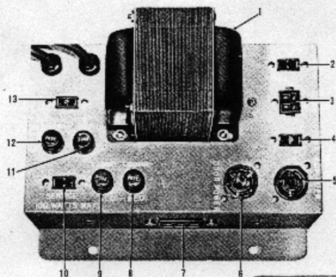
No. 30520-A Power Distribution Panel Assembly
