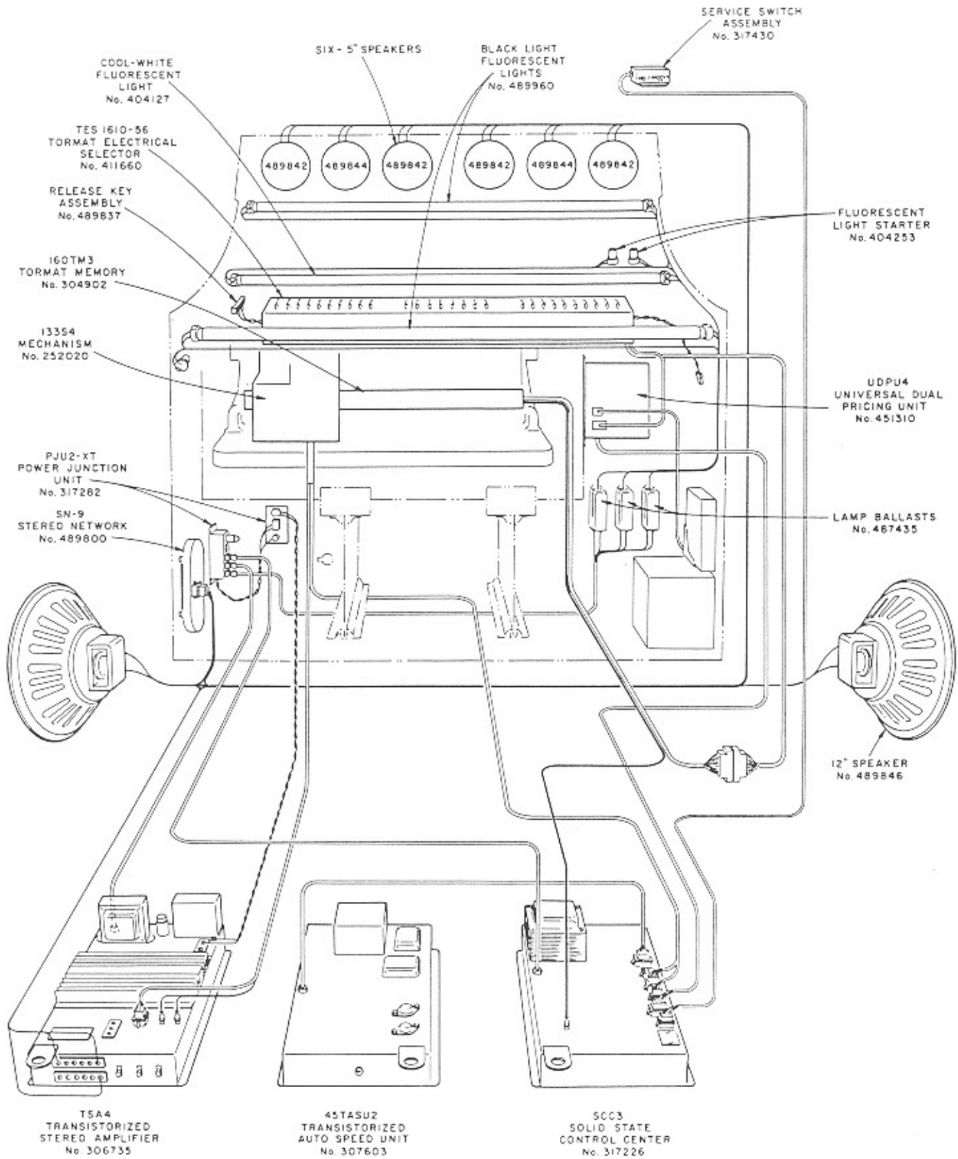
Cabinet Cabling Diagram, PFEA1U Model.
