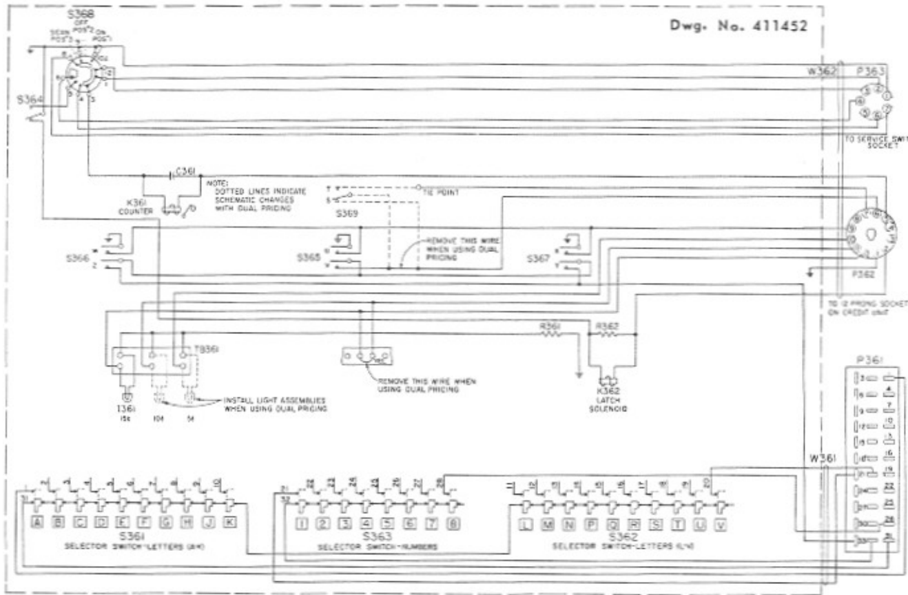
Schematic Diagram for Tormat Electrical Selector, Type TES168.
