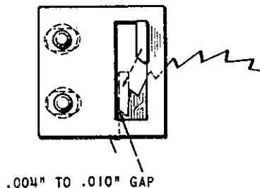
FIGURE 7. PAWL &amp; GUIDE GAP
