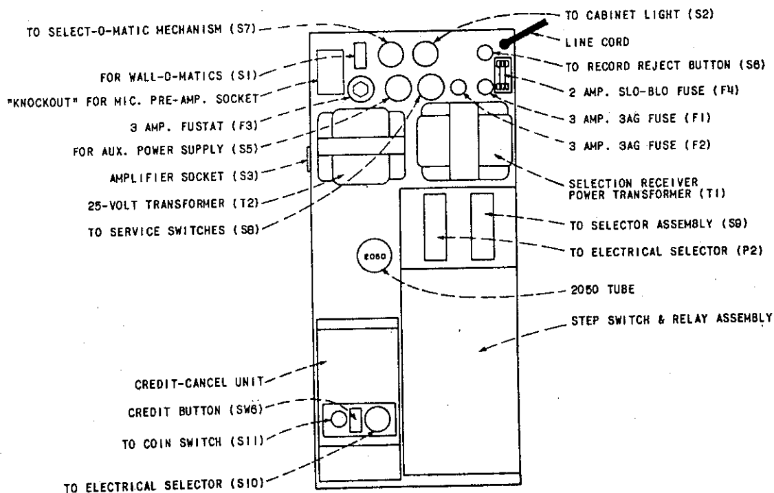
FIGURE 1. TOP VIEW OF SELECTION RECEIVER
