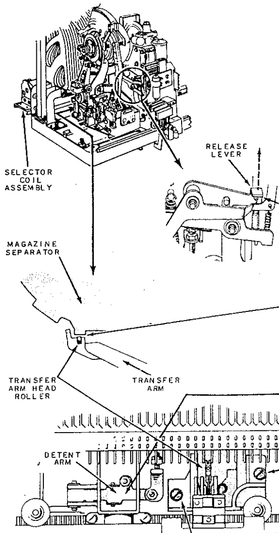
REAR VIEW WITH SELECTOR COIL ASSEMBLY REMOVED
