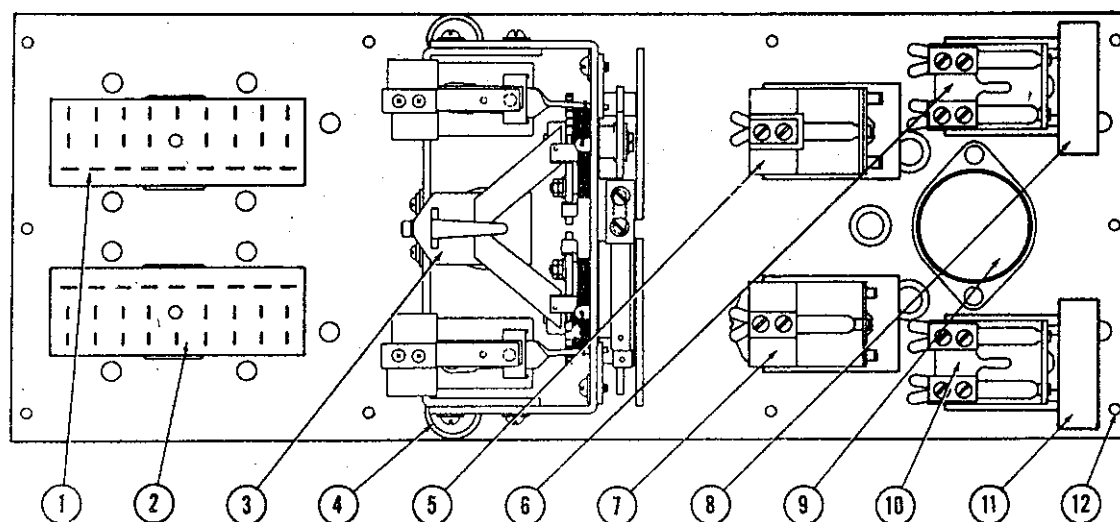
Figure 14. #303283 Step Switch &amp; Relay Assembly
