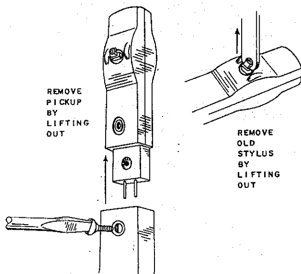
FIGURE 7. STYLUS REMOVAL
