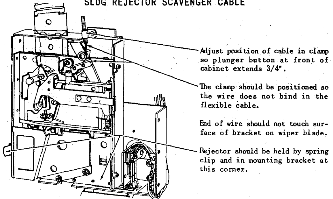
FIGURE 10. CABLE ADJUSTMENT
