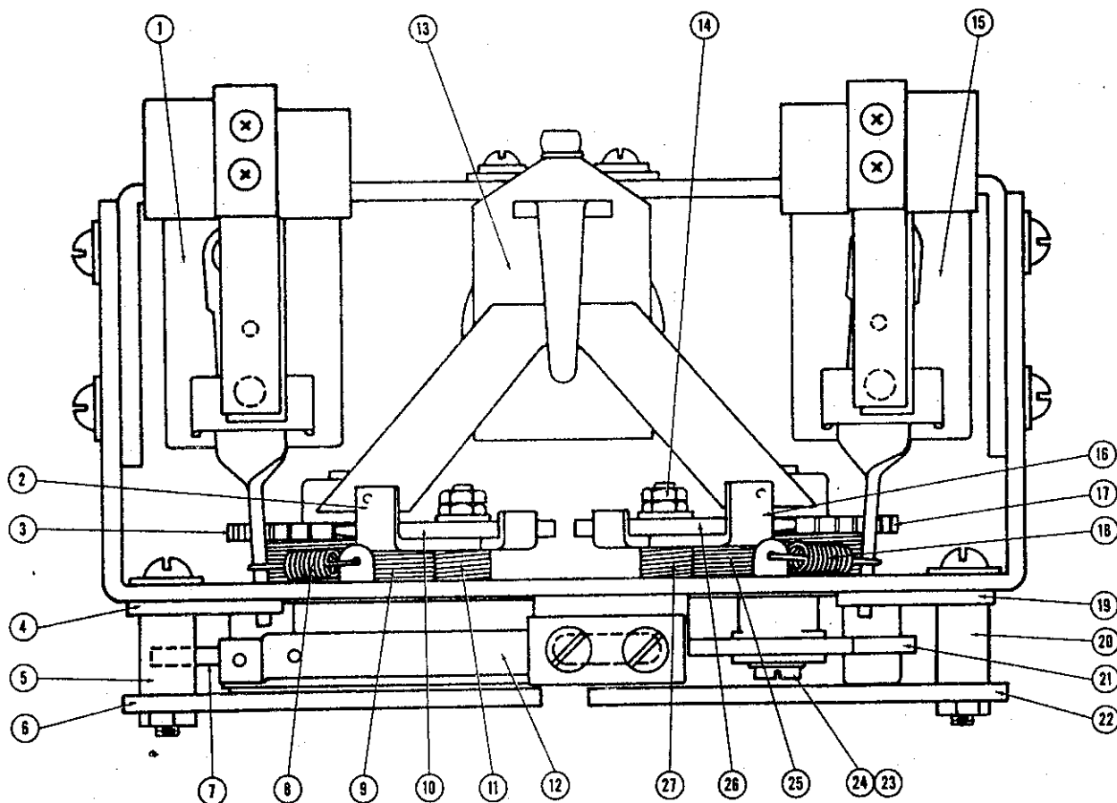
FIG. 15. #303063 STEPPER ASSEMBLY
