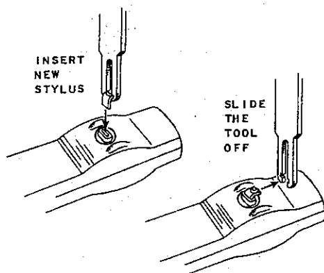
FIGURE 8. STYLUS REPLACEMENT
