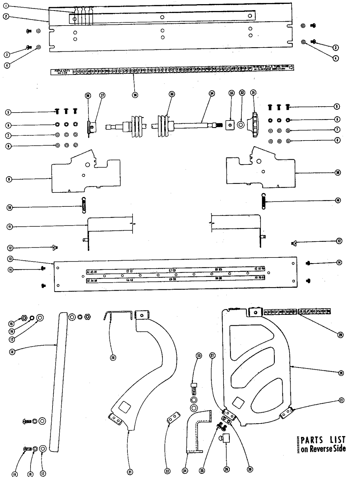
POPULARITY METER & MAGAZINE ASSEMBLY
