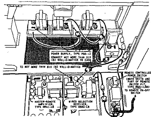
FIGURE 2. SHOWING PLACEMENT OF ACCESSORIES
