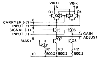
IC-2, MC1496N
