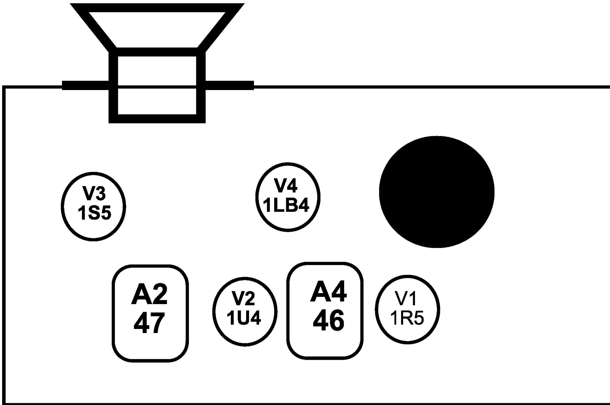
Arvin 244-P Chassis: RE-259 Bottom View
