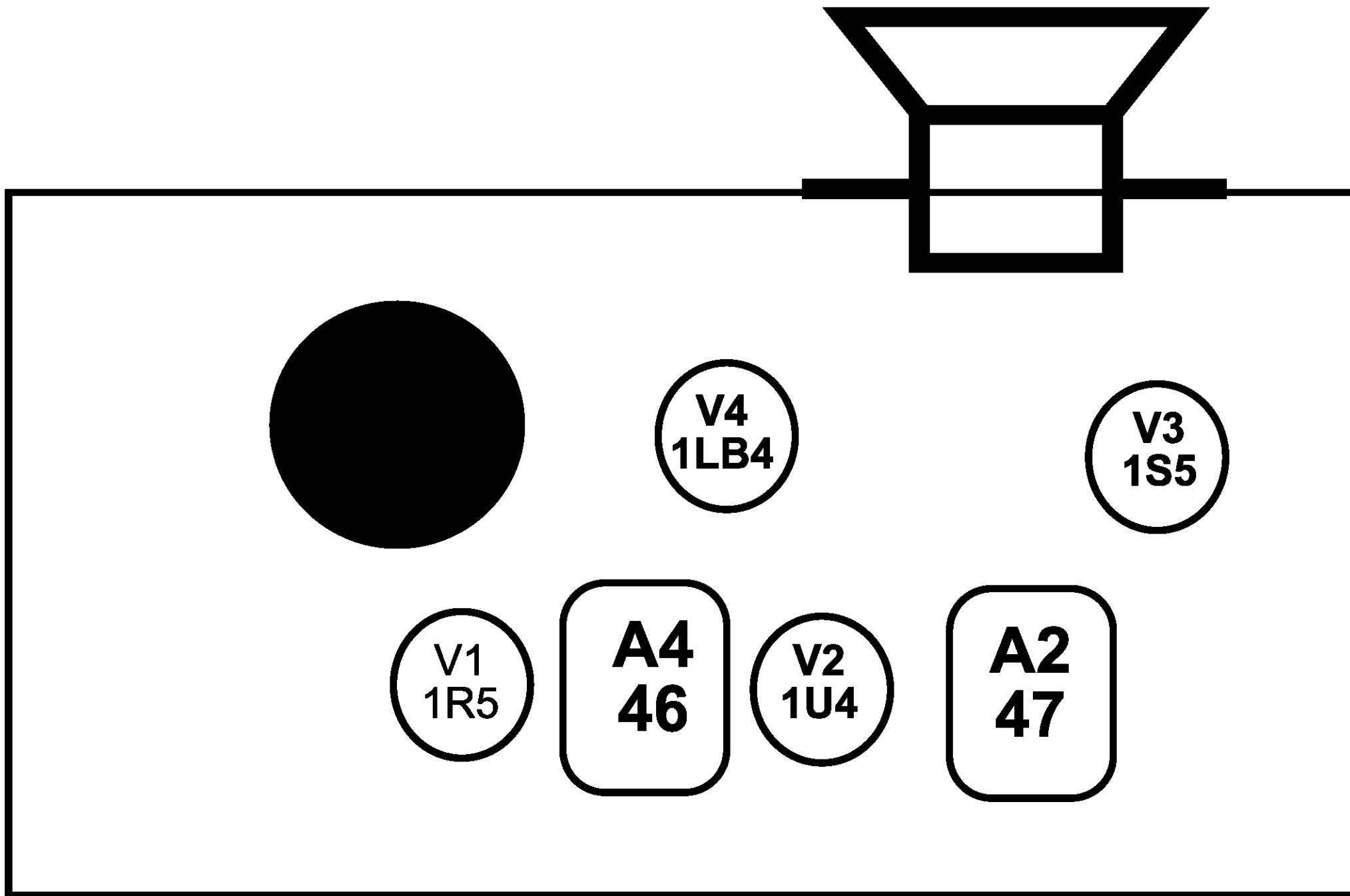
Arvin 244-P Chassis: RE-259 Top View
