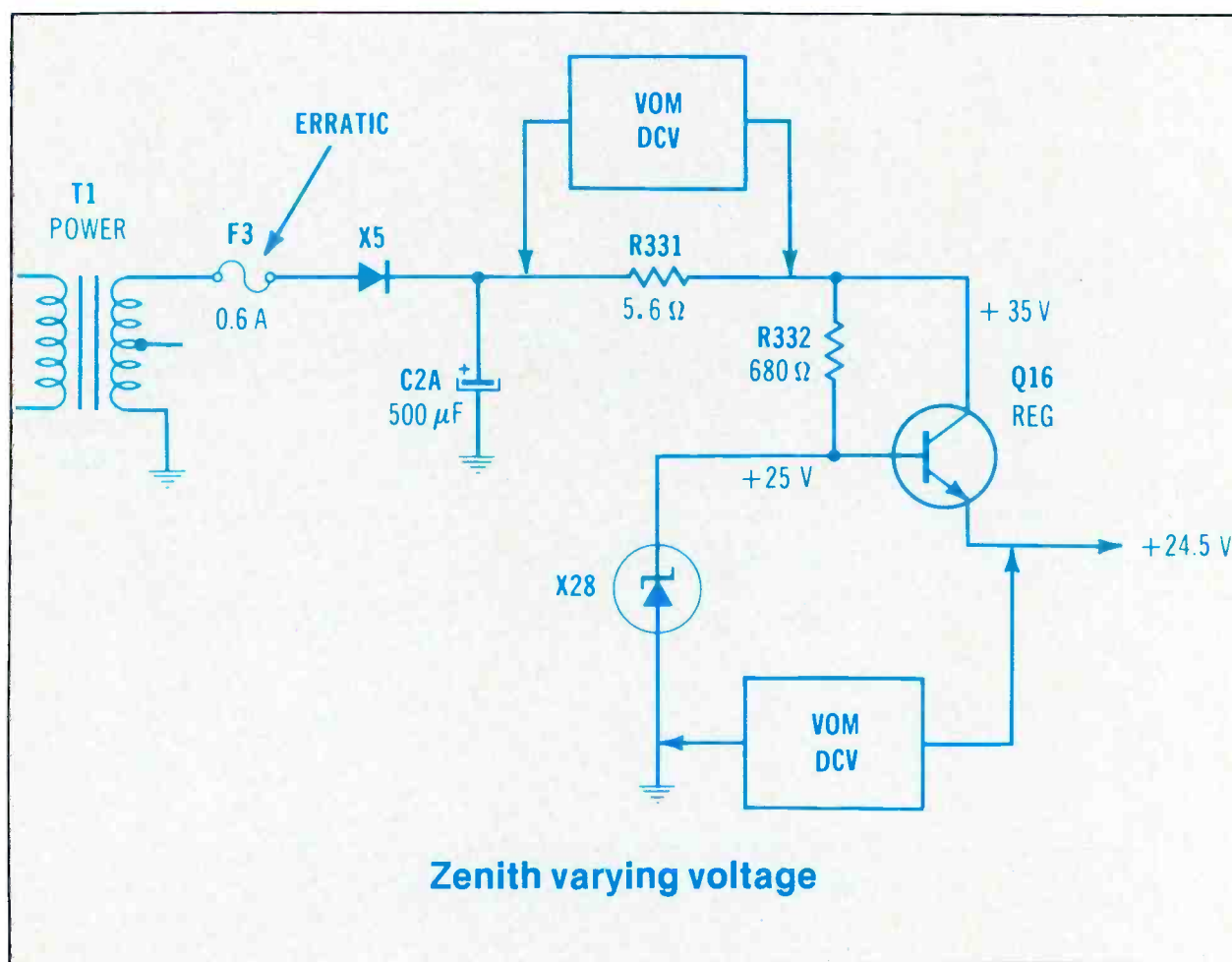
Figure 4 A reduction of supply voltage when the symptom occurred led the technician to this method of monitoring the current and voltage of the +24V supply.
