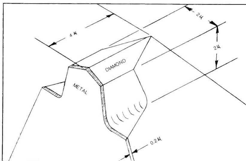
Figure 4. The stylus is made of diamond with a thin metal electrode on one face. The end of the stylus is shaped to fit the groove and long enough to cover several of the longest recorded waves. The sides are cut away to provide a "keel-lapped" shape which gives long-play life as the end of the stylus is worn away. The end of the metal electrode is one plate of a capacitor, the disk is the other plate, which varies in value as the disk is played and provides the read-out signal.
