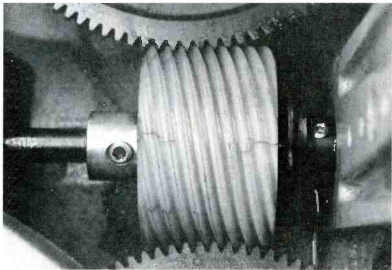
Figure 9 The effects of correct and improper lubrication of the main worm gear are shown. Top, a correctly lubricated (with Bell & Howell 070043 grease) worm gear has an even coating of grease. The gear is not cracked or chipped. Above, a similar worm gear having insufficient, infrequent or incorrect lubrication is likely to have cracks requiring replacement of the gear.
