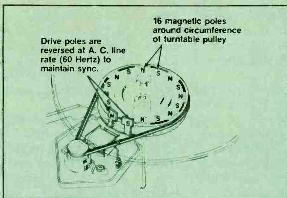
Figure 9. The major drive components in the disc rotating system. Included are the ac motor, compliant rubber belt, drive poles and magnetic strip.
