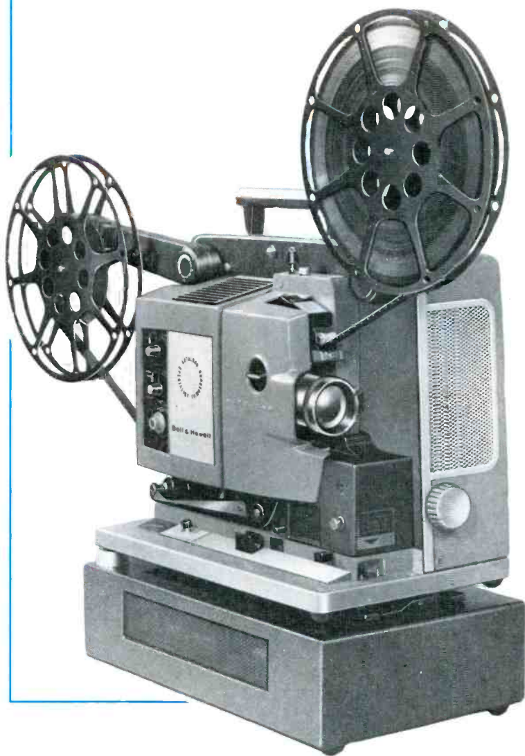
Figure 4 A Bell & Howell model 566T is shown ready to project a sound film. This is an auto-loading late-production 500-series. (Courtesy of Bell & Howell)
