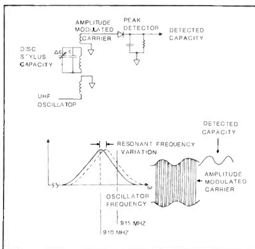
Figure 5. Disk-stylus capacitance is made part of a circuit resonant at 910MHz. As the capacitance changes, the resonant frequency changes, giving rise to a variation in the response of the circuit to a 915MHz signal and providing amplitude modulation of this signal. The modulation is stripped off by a diode detector to provide a voltage that rises and falls as the disk surface rises and falls under the stylus.
