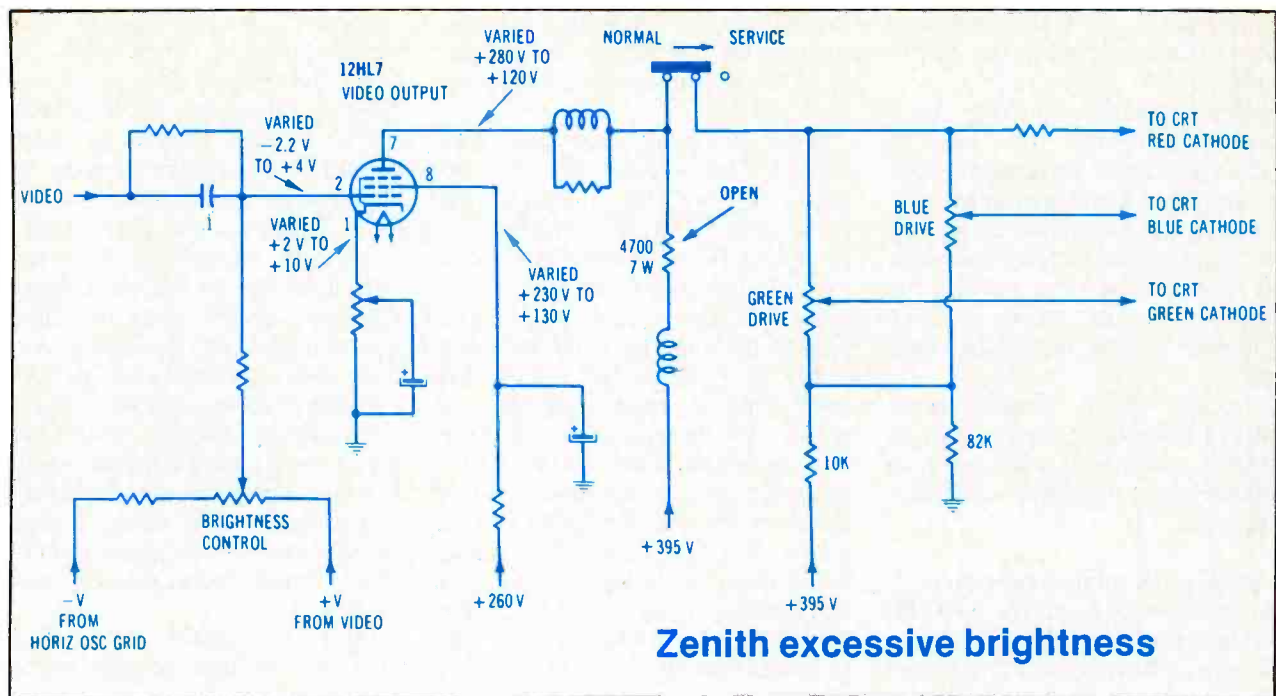
Figure 5 Several voltage measurements and intuition enabled an experienced technician to find the bad component in a very short time.
