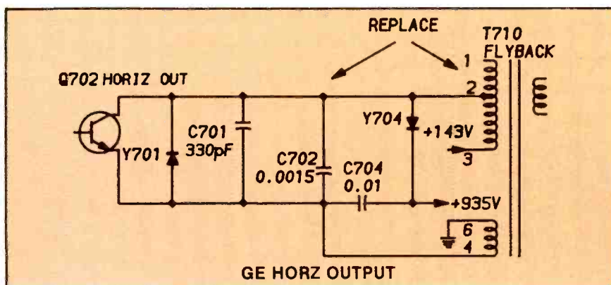
Figure 6. Replacement of the T710 flyback and the C702 retrace-tuning capacitor eliminated the problems of foldover in the center followed by loss of picture. This model uses a regulated power transformer, so it does not require a regulated power supply nor a start-up supply. Neither does it have a recognizable shutdown circuit.
