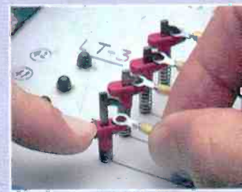
Nail-Clip Harnessing
