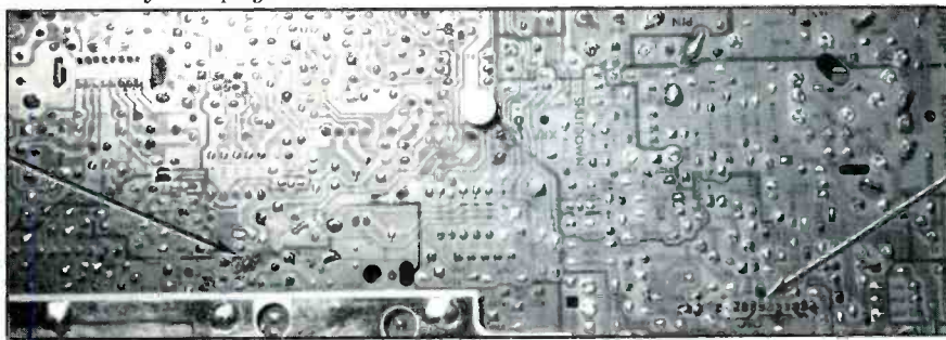
Melted wiring and burned areas of the circuit board are common after lightning has reached a TV receiver via the power line or antenna lead. Check all circuit boards carefully for such damage.
