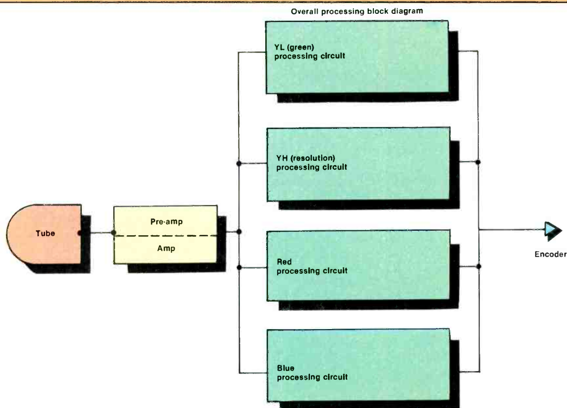
Figure 4. The color components are matrixed to create the complete range of colors.
