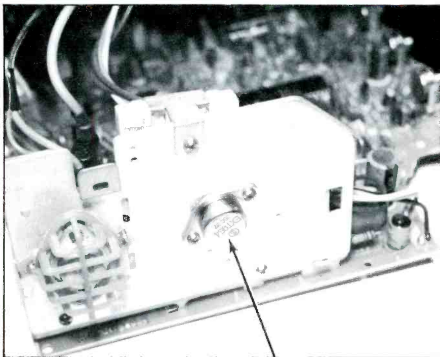
Figure 1. Excessive amplitude of pulses from the flyback of a 13F22 Sharp (Photofact 2045-2) triggers the safety circuit inside IC501, which then eliminates the horizontal oscillator output signal. Without a drive signal to the Q601 horizontal-driver transistor, the horizontal-sweep circuit cannot operate. To disconnect the safety circuit during short tests, unsolder the ZD651 anode lead. After all repairs and adjustments have been made, temporarily connect a 6.8k resistor between testpoint TP651 and the +33V source at the D503 cathode. Instantly, the receiver should become dead (in shutdown). Turn off the power for a minute, remove the 6.8k resistor, and then switch it on again. The receiver now should operate. Don't consider the test completed until the receiver's safety-circuit operation has been checked and found to be correct.
