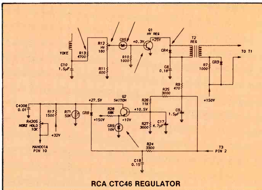
Figure 4. Arrows point to the components most likely to produce excessive high voltage in RCA CTC46A chassis (Photofact 1278-3). Suspect R13, R12, CR5, CR4, Q1 and T2 if the high voltage cannot be adjusted. Or, check Q2 and CR9 if the HV can be adjusted correctly, but the horizontal hold cannot be locked. In this older model, excessive HV or a shutdown-circuit defect changes the horizontal frequency so much that the hold control cannot lock the picture.
