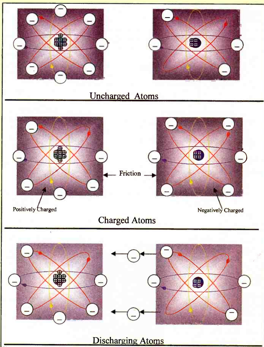
Figure 1. When two non-conductive materials are rubbed together to create friction, an imbalance occurs between the atoms of both materials. This imbalance leaves one material lacking electrons (positively charged) and the other material with an excess of electrons (negatively charged)
