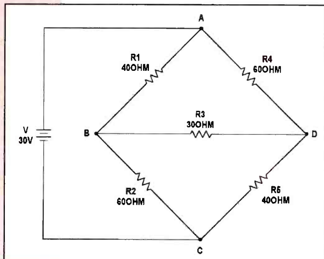
Figure 1. This is the student's drawing, showing his conception of the currents through the circuit.
