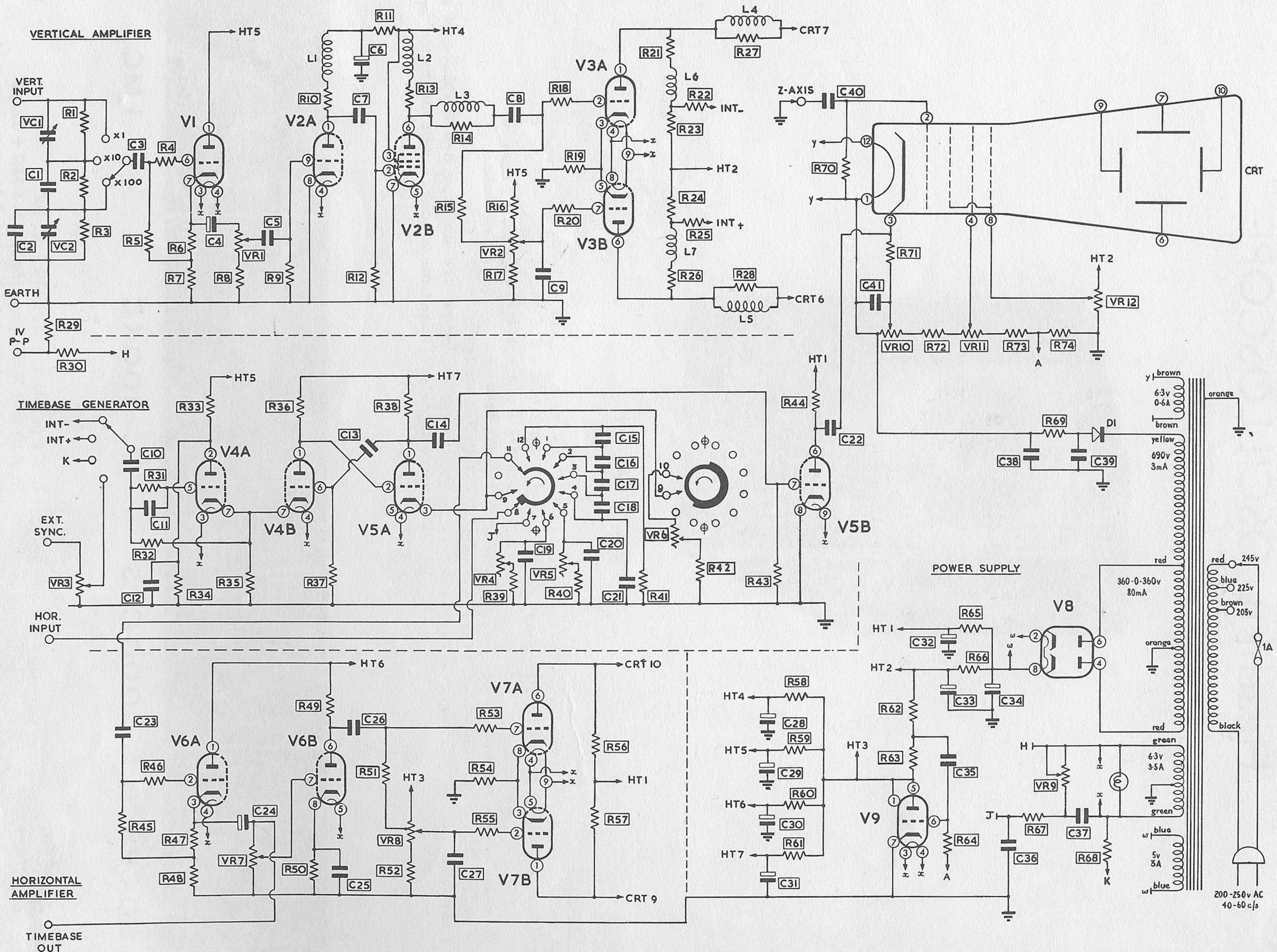
CIRCUIT DIAGRAM OF THE HEATHKIT LABORATORY and GENERAL PURPOSE OSCILLOSCOPE Model IO-12U
