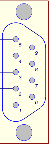
Front View (Pin)
