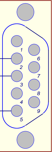
Front View (Socket)
